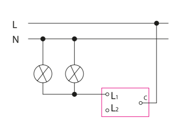
Dimmer
