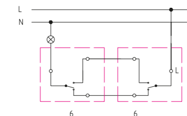
Two-way switches (cooperation)
