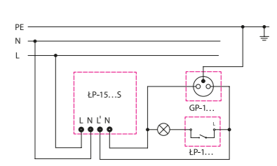
Hotel switch
