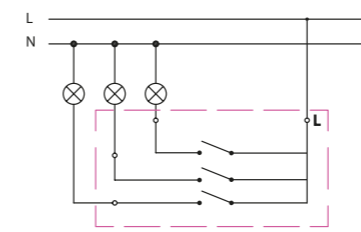
Triple switch
