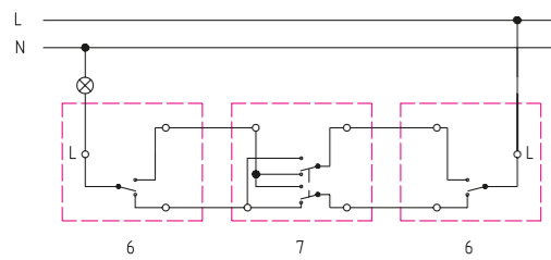
Intermediate switch (cooperation with two-way switches)
