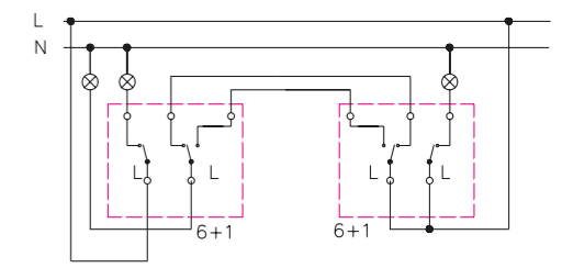
Cooperation of two-way and single pole switches
