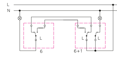
Cooperation of two-way and single pole switch with two-way switch
