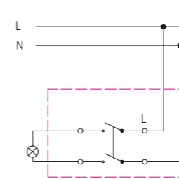
Control switch
